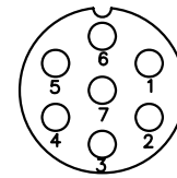
7 PIN
